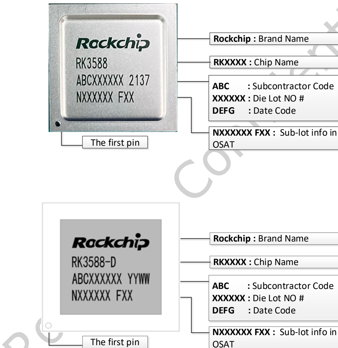
Fig. 2-1 Package definition
